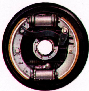
Rear Brake
